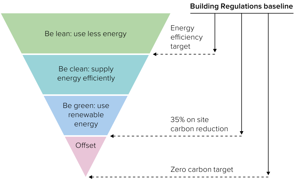
Figure 30. Energy hierarchy
